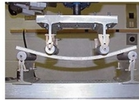
Bending Test
